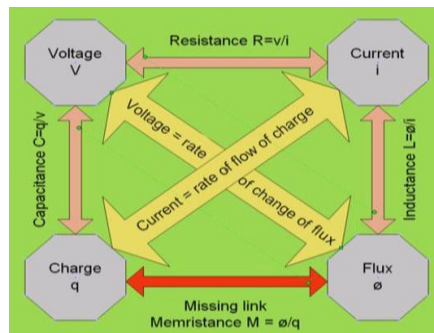
Figure 1: Fundamental circuit element relations
