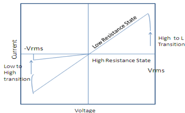
Figure 4 : I-V characteristic (Hysteresis Loop)
