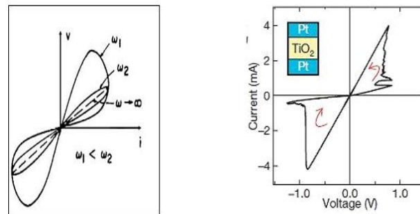
Figure 5: (a) Chua's Predicted Model results and (b) HP Lab Model results
