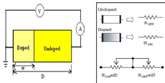
Figure 6 : Memristor Device Structure and Model
